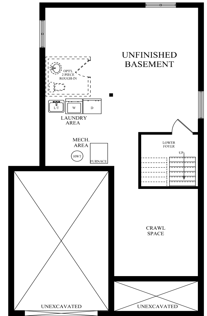
BASEMENT
