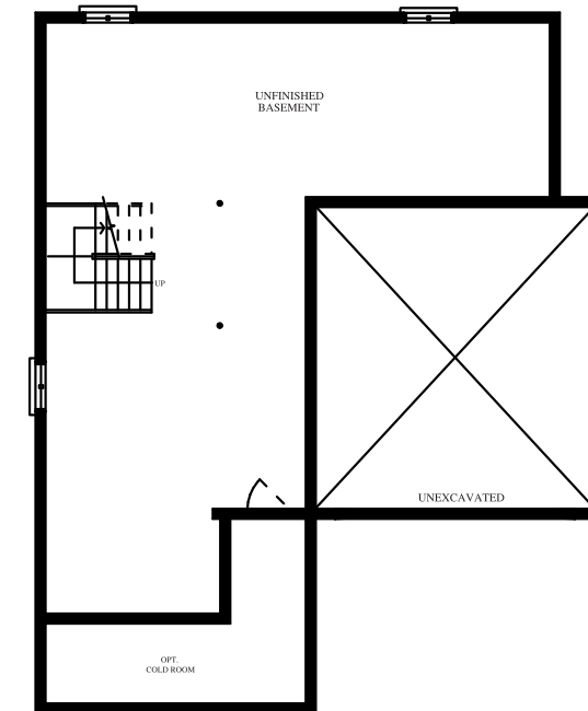
BASEMENT
