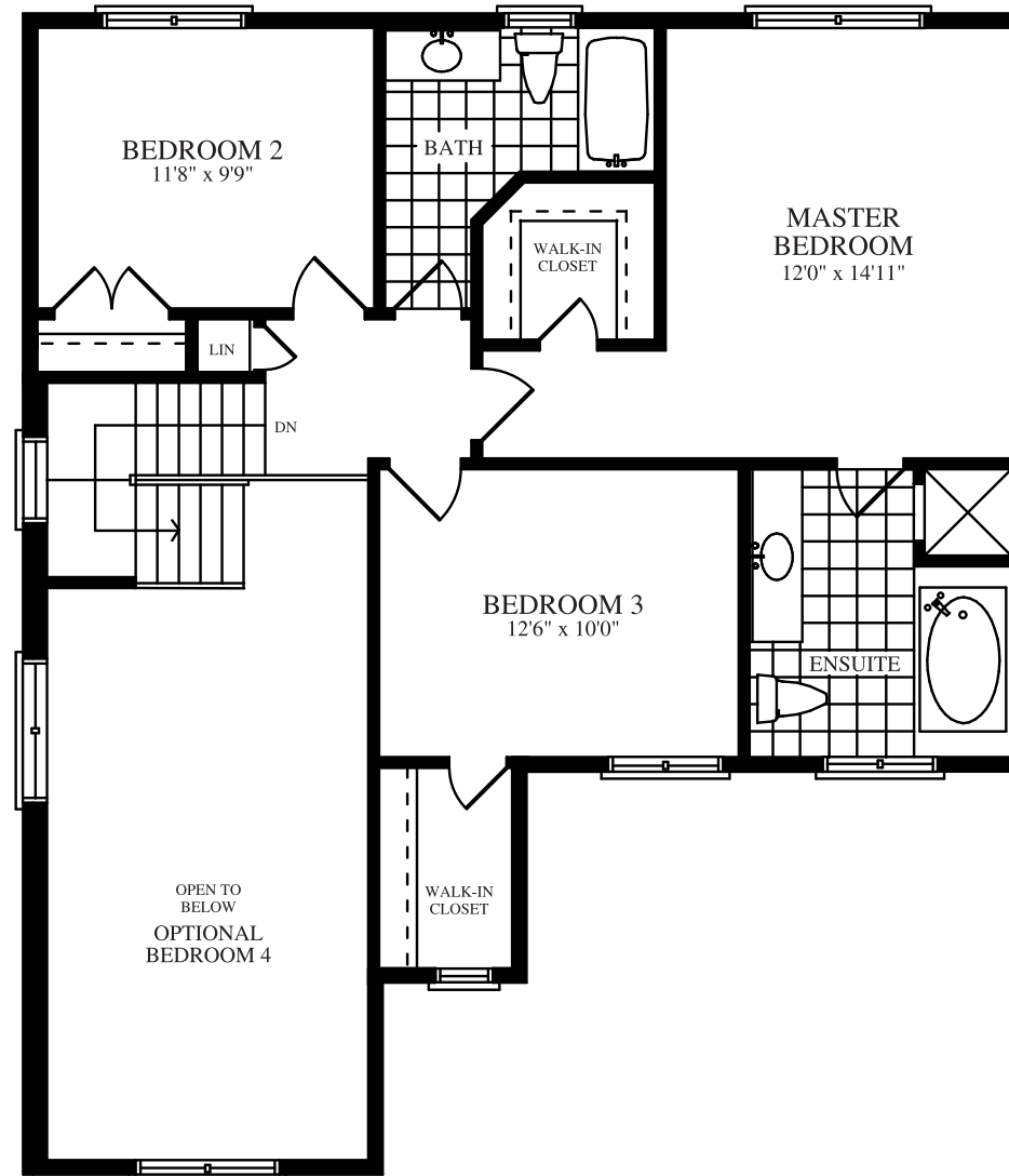
SECOND FLOOR
