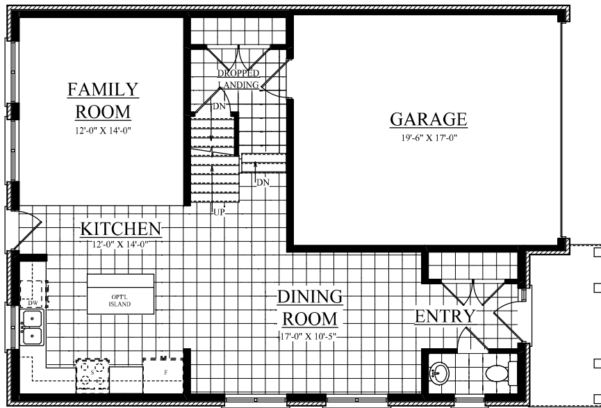
MAIN FLOOR 855 SQ. FT.
