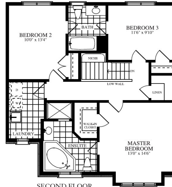
SECOND FLOOR 3 BEDROOM
