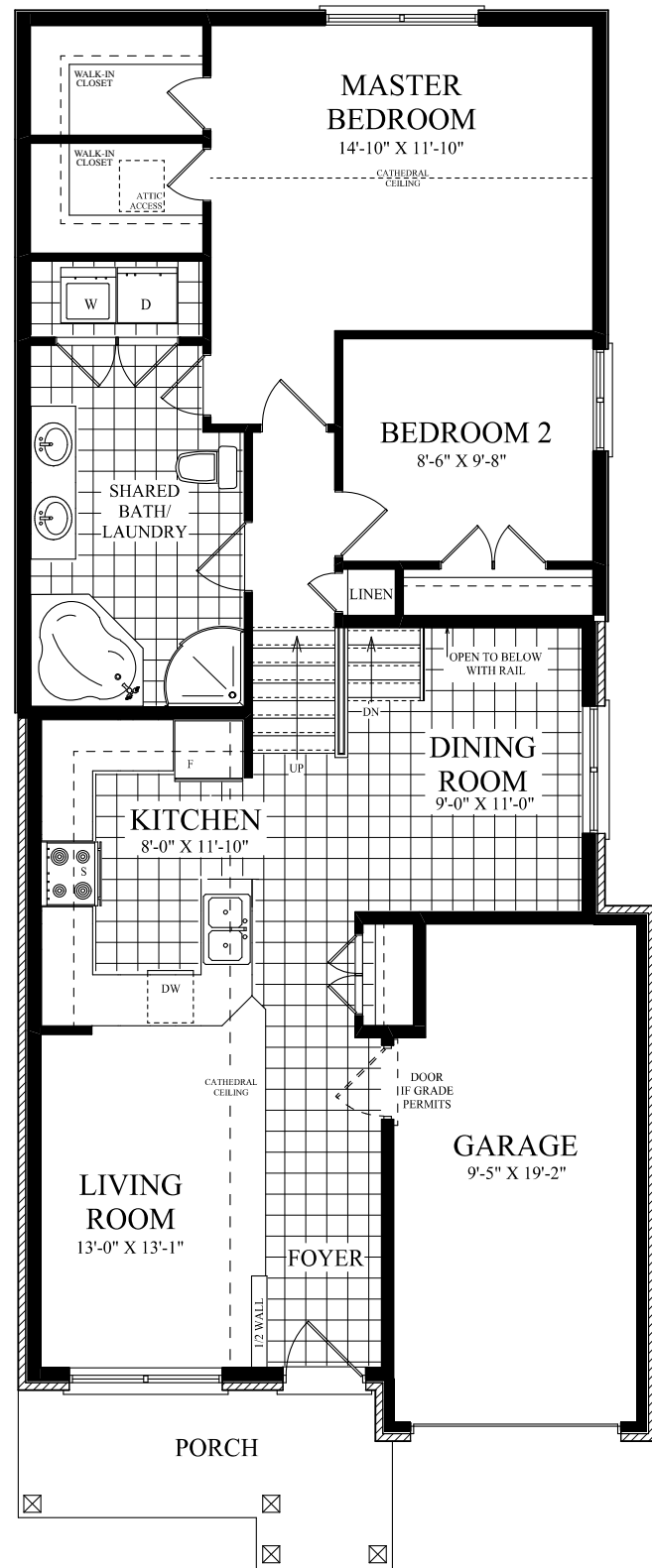
MAIN FLOOR
