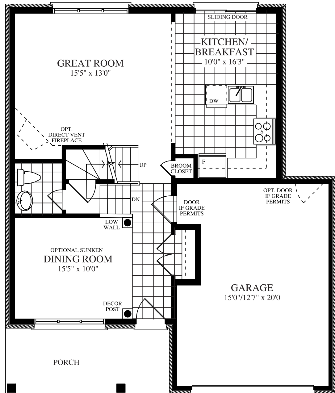
GROUND FLOOR
