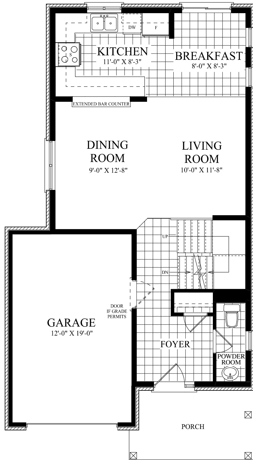
MAIN FLOOR
